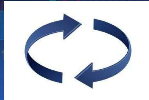
Reverse Trading
